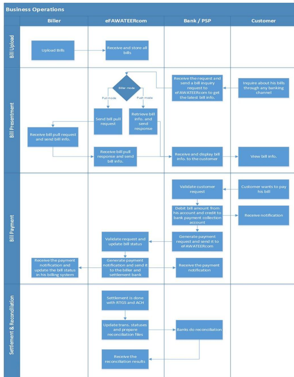
Figure 9: Business Process Operation
