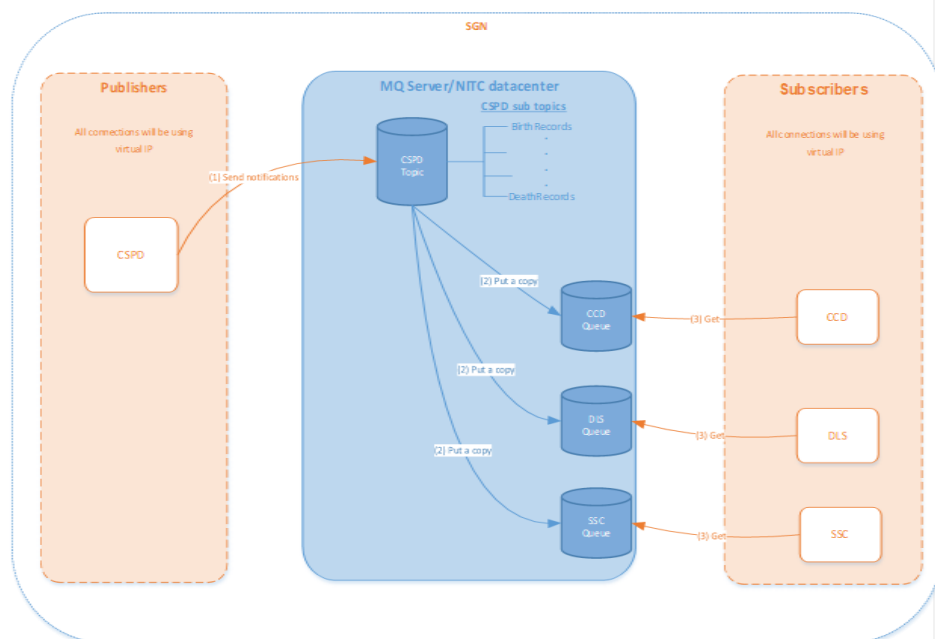
Figure 7: Publish-Subscribe Business Case
